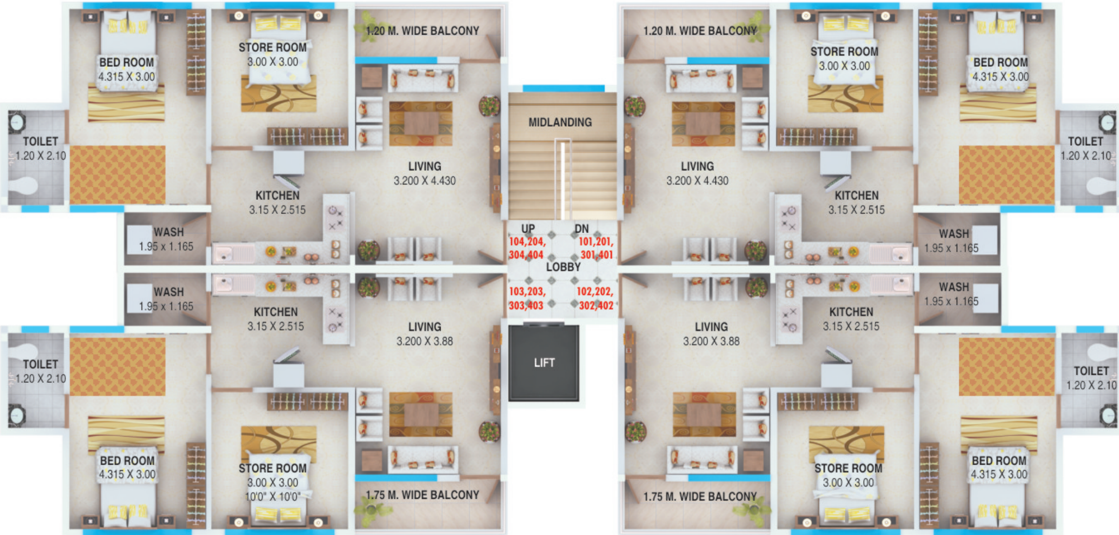
FIRST TO FOURTH FLOOR PLAN
